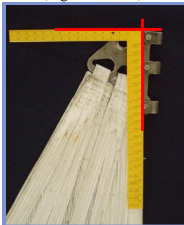
Figure K.2.1.5 Mainsail head point.
