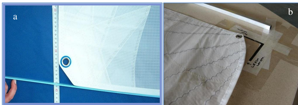
Figure K.2.1.1 Clew point definition.
