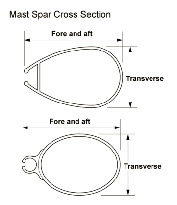
Spar section measurement.
