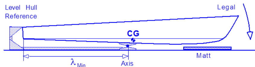
Figure H.4.2 Test to establish that the CG is forward of \lambda_{Min} .
