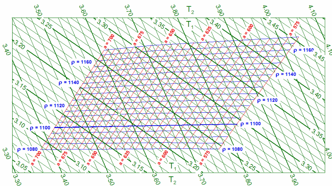
Figure H.4.1.3 The Finn graph introduced by Gilbert Lamboley for determining “a” and “p” from the periods T_1 and T_2 , given that b = 200.0 mm.
