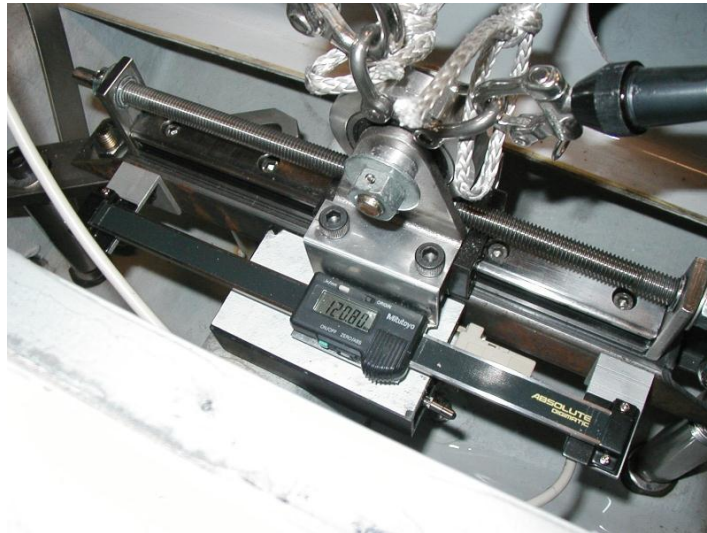
Figure H.4.7.2 The 2004 tilt swing system installed on the keel bolts of an Yngling. The swing bearing is mounted on a precision rail and the position read on the electronic scale. The box below the “rail scale” is the inclinometer. The roller bearing and the shackles for the support and steady lines of the suspension can be seen at the top of the photograph.
