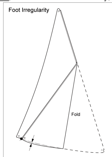
Figure K.2.4.5 Foot irregularity.
