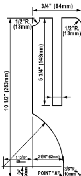
Centreboard Thickness Measuring Device
