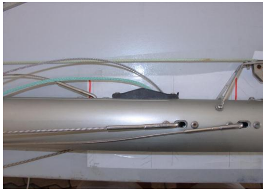
Rigging points: shroud, forestay, trapeze. Heights to be measured from MDP.
