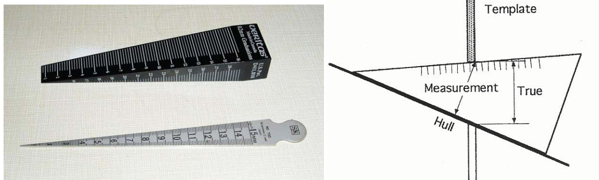
Figure F.4.6 Two types of wedge gauge and the error in gap measurement.
