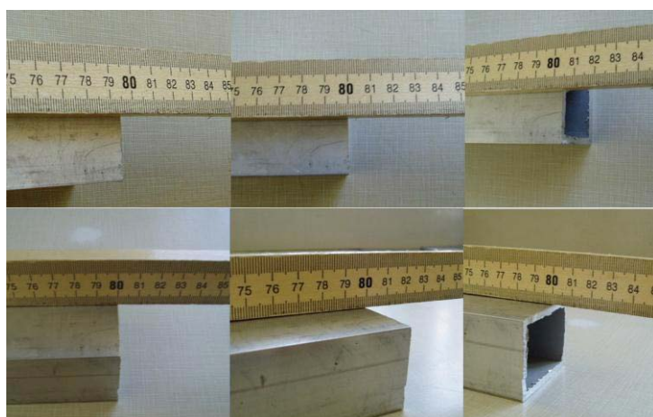
Figure F.4.3 The parallax error when sighting a non-contiguous scale
